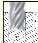
Slotting
