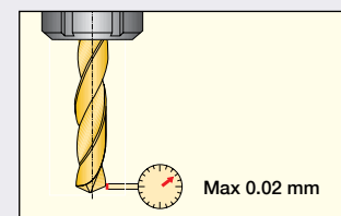
Rotating Drill
